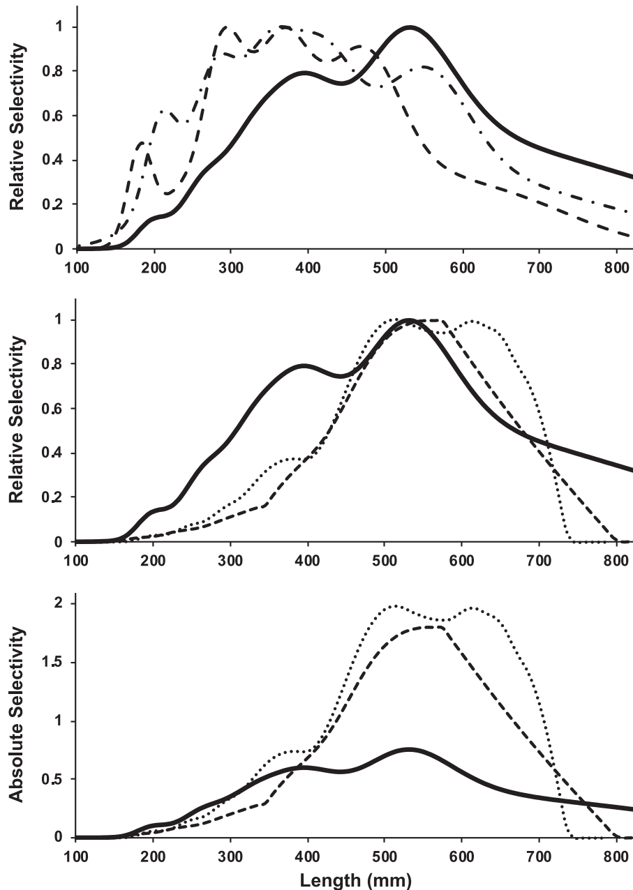
FIGURE 8. Estimated relative ( S_L ) and absolute selectivity ( \zeta_L ) by Walleye total length (mm) for Minnesota's standard gill net by using the statistical assessment model (dark line) compared with the other models. The top panel includes the relative selectivities from the models from Vandergoot et al. (2011), shown by the long dashed line, and Shoup and Ryswyk (2016), shown by the long dash-dot line. The middle and lower panels include selectivities from the models from Hamley and Regier (1973), shown by the dotted line, and Anderson (1998), shown by the dashed line.
